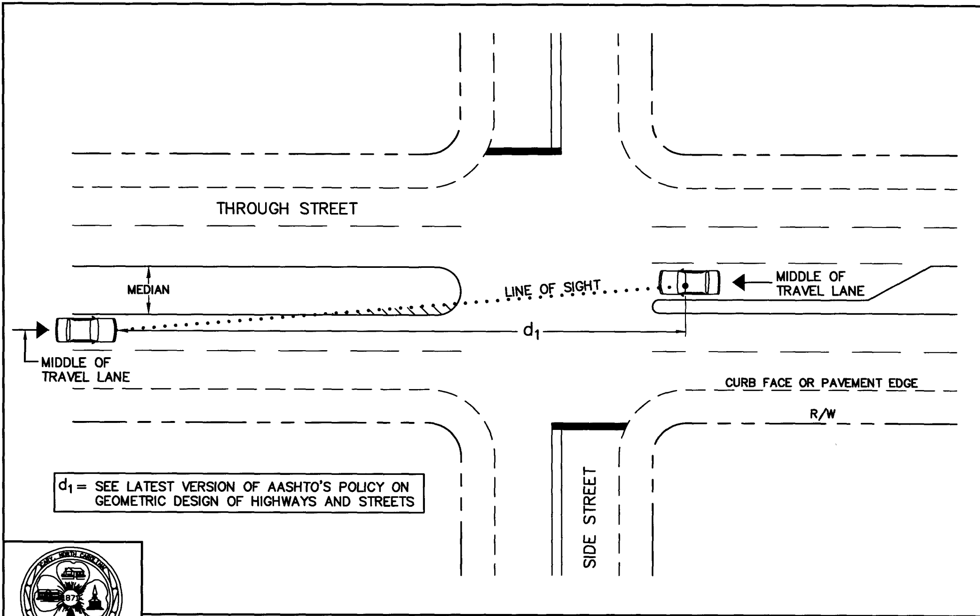
INTERSECTION SIGHT DISTANCE FOR LEFT TURN MOVEMENTS FROM THROUGH STREET
