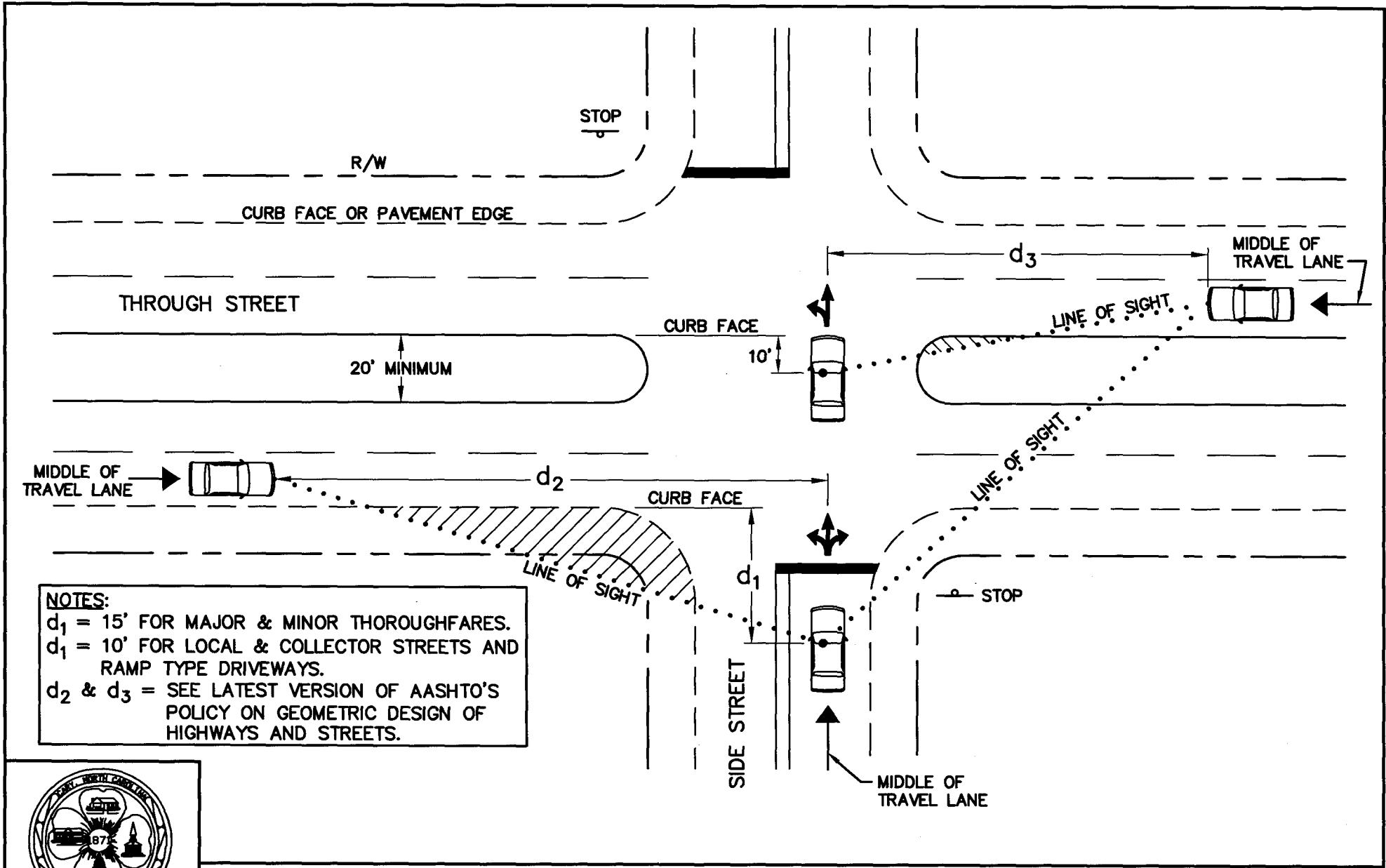
INTERSECTION SIGHT DISTANCE FOR LEFT, RIGHT, AND THROUGH MOVEMENTS FROM THE SIDE STREET
