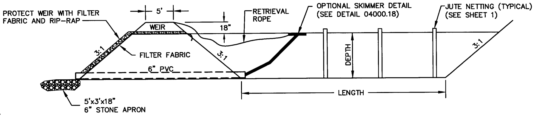
WEIR DETAIL
