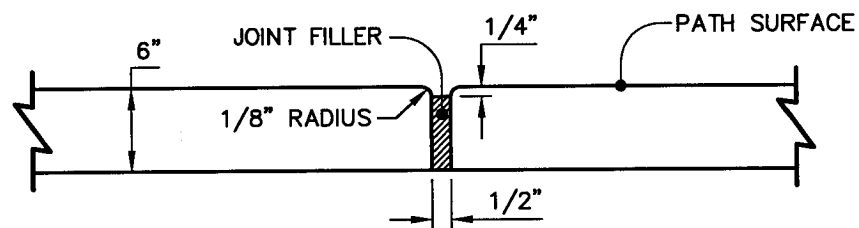
TRANSVERSE EXPANSION JOINT
