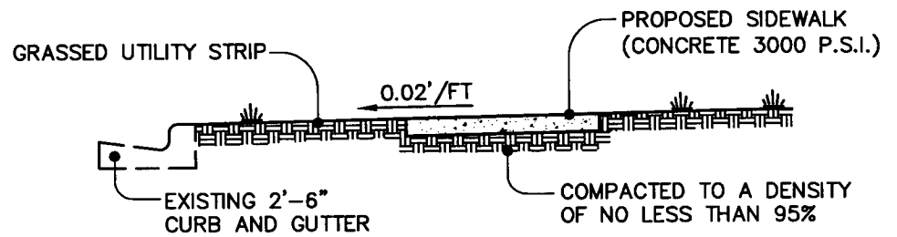
TYPICAL SECTION
