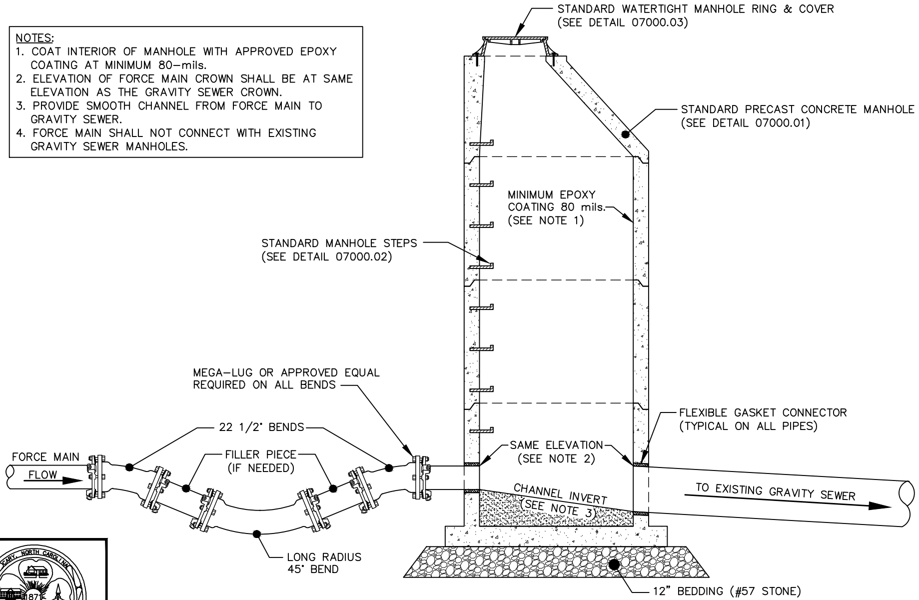
FORCE MAIN DISCHARGE MANHOLE, TYPE 2 FLAT OR DOWNWARD SLOPING FORCE MAIN
