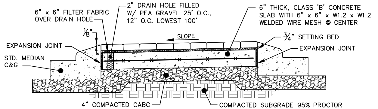
BRICK PAVER MEDIAN SECTION VIEW
