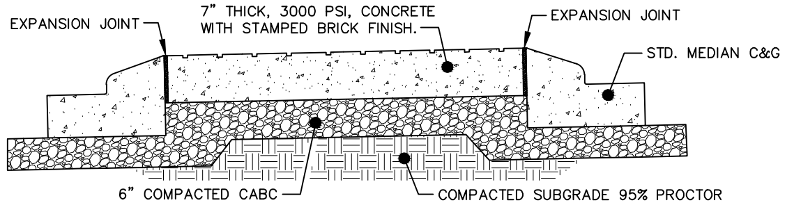
STAMPED CONCRETE MEDIAN SECTION VIEW
