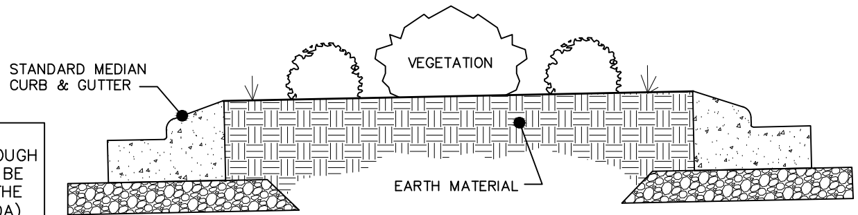
LANDSCAPED MEDIAN SECTION VIEW
